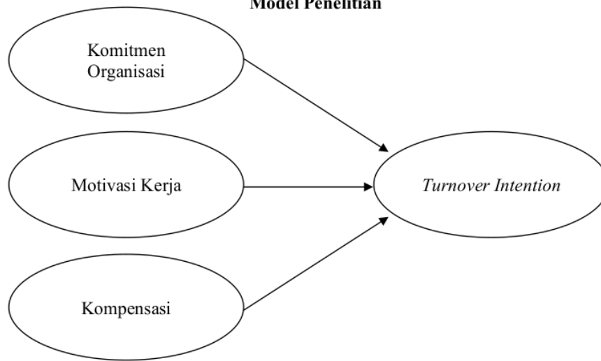
Gambar 3.1 Model Penelitian
