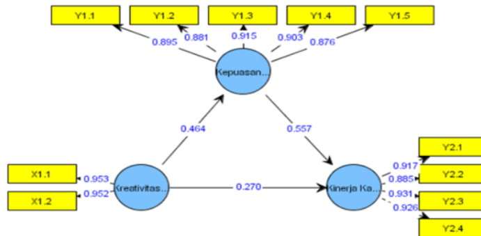
Gambar 2. Hasil Output PLS
