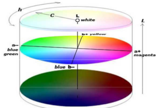
Gambar 2. CIELAB Color Model. 4
