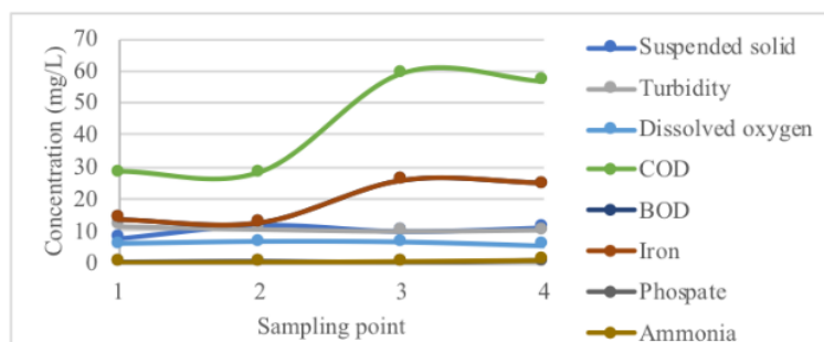
Figure 2 Concentration trend of physicochemical parameters along the sampling points
