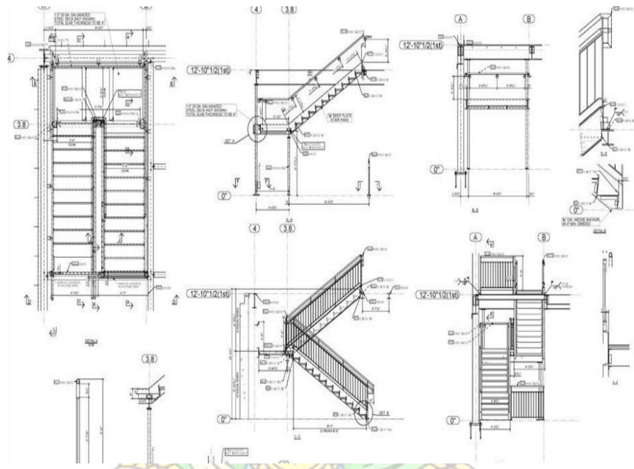
Gambar 2.8 Shop Drawing
