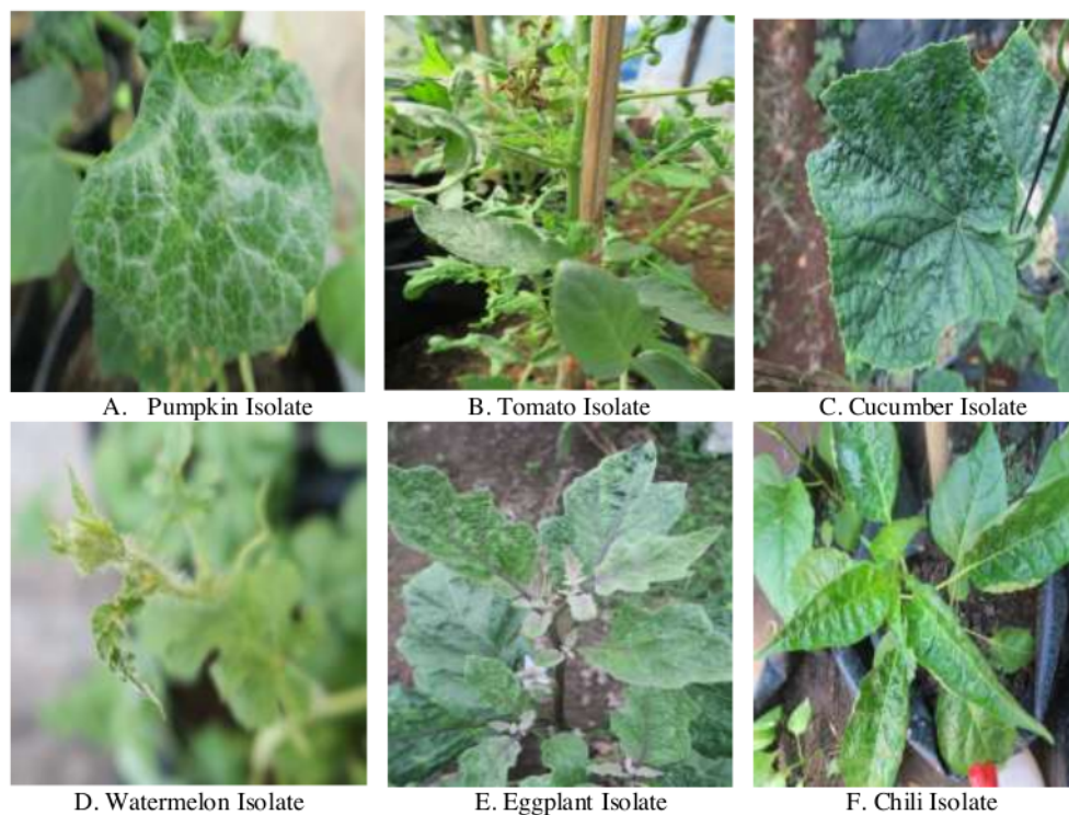
Figure 2. CMV-Bali isolates
