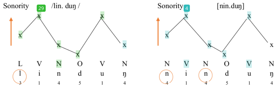
Figure 7. Reverse ordering sonority
